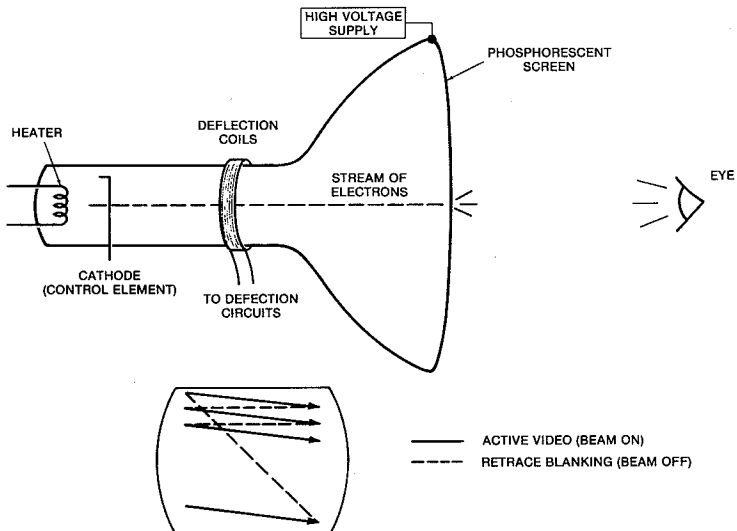
Fig. 8-1. Cathode-ray tube.
